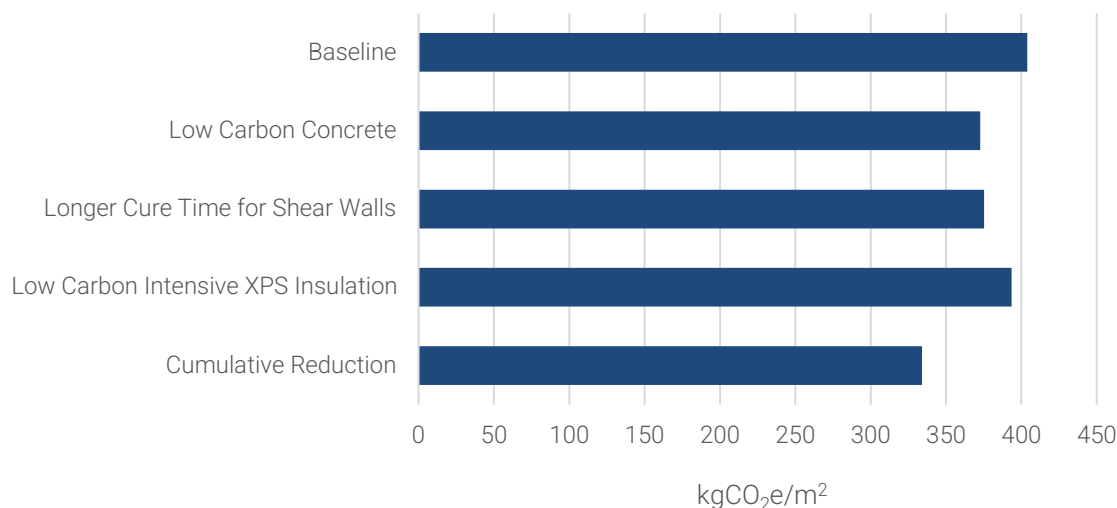
Figure 19– Embodied Carbon Reduction Summary Graph
