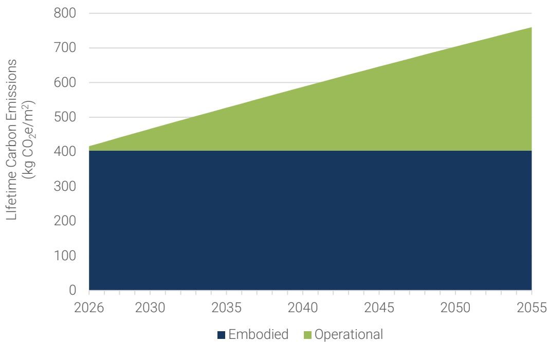
Figure 14 - Embodied versus Operational Carbon
